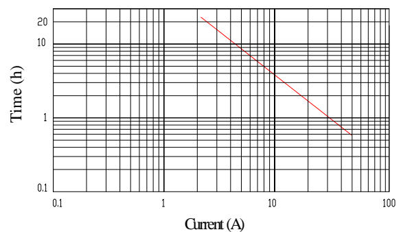
DISCHARGE CURRENT VS TIME 25° C(77° F)
