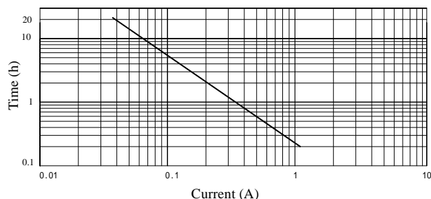
DISCHARGE CURRENT V'S TIME 25° C(77° F)
